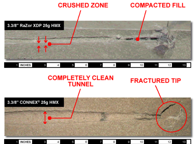
Figure 1: Comparison of perforating tunnels in stressed Berea sandstone produced using a conventional deep-penetrating shaped charge (top) and a reactive shaped charge (bottom)
