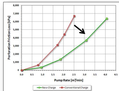
Figure 2: Step rate test data showing reduction in perforation friction as a result of using reactive shaped charges.
