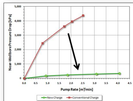
Figure 3: Step rate test data showing near elimination of near-wellbore pressure drop (“tortuosity”) as a result of using reactive shaped charges.
