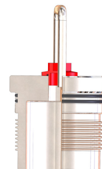
CARRIER (GUN) PROTECTOR EQUIPPED WITH MELT PLUG AND O-RINGS
