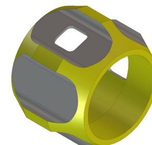
6-1/4" OD EXTENDED RING CENTRALIZER GN-RH475-R625-EXT
