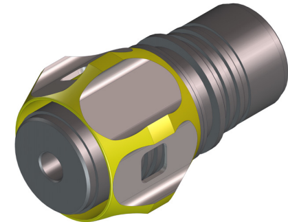
CENTRALIZING TANDEM SUB GN-R45-0021HB
