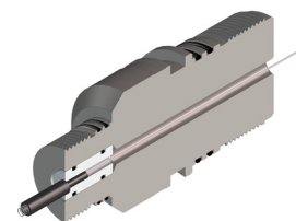
SPRING CONTACT ASSEMBLY GN-E00-0020 (4-1/2" OD TOP SUB SHOWN FOR REFERENCE ONLY)
