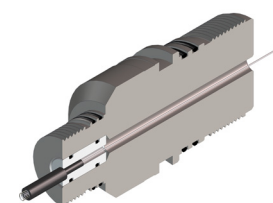
WIRELINE INSERT GN-E00-0011
