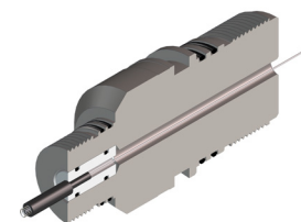
WIRELINE INSERT GN-E00-0011 SPRING CONTACT ASSEMBLY GN-E00-0020 (4-1/2" OD TOP SUB SHOWN FOR REFERENCE ONLY)
