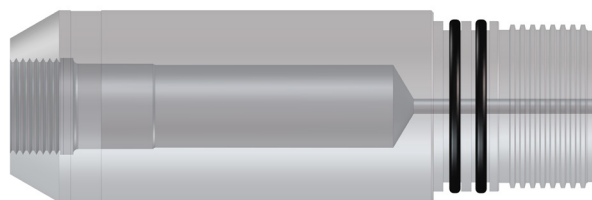
STANDARD 1-3/16" 12P GO STYLE TEAR DROP UPPER HEAD CONNECTION.
