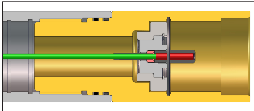
TRANSFER SUB, GN-R33-0060
