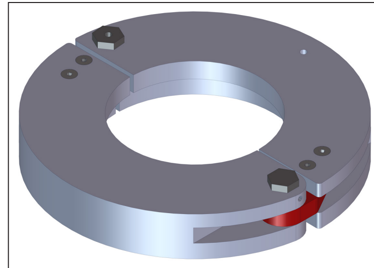
6.75" LIFTING CLAMP ASSY TC-LC-0675-0000 (SHOWN)
