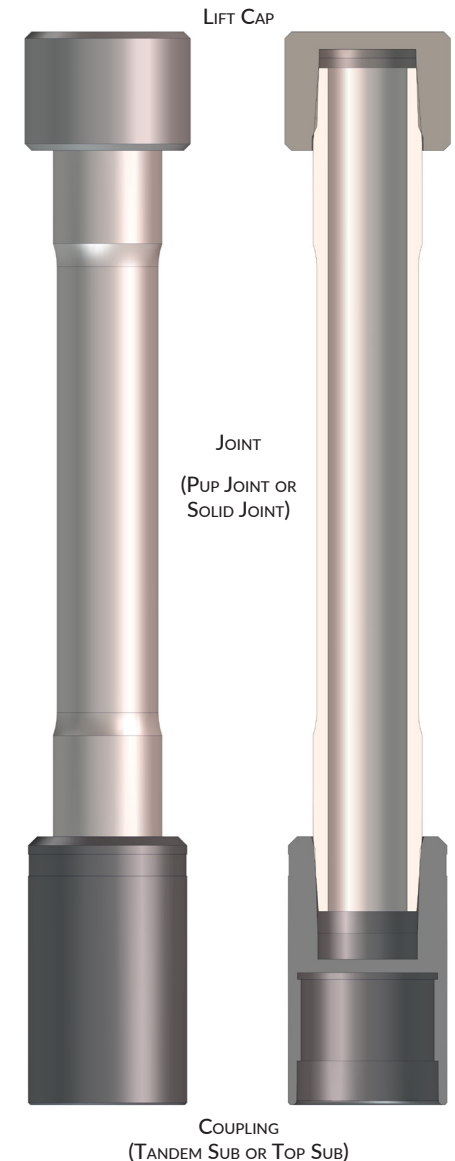
LIFT SUB ASSEMBLY, 4-1/2" & 4-5/8" TANDEM TC-LT45-000 (SHOWN)
